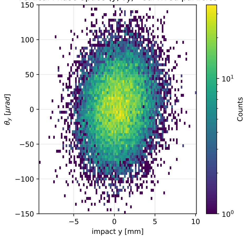
Vertical Phase Space (y, theta_y) - survived particles
